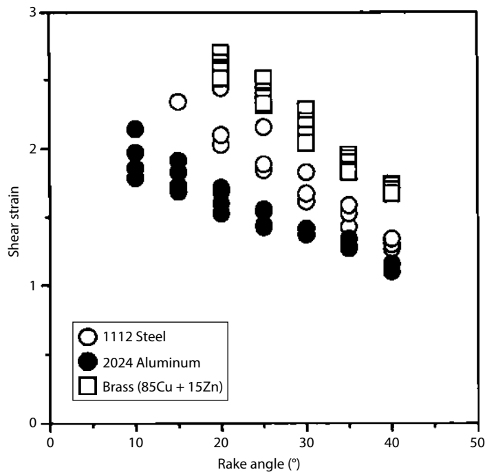
FIGURE 6.16 Shear strain when cutting steel, aluminum, and brass with tools with varying rake angles. (Data of Eggleston, D.M. et al., ASME J. Eng. Ind. , 81, 263, 1959.)
