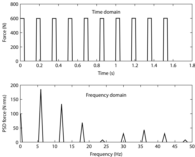
FIGURE 12.8 Step Forcing Function and PSD simulating a SDOF system of a flymill single insert rotating at 360 rpm during in a ½ slot. (Courtesy of D3 Vibrations Inc., Royal Oak, MI.)
