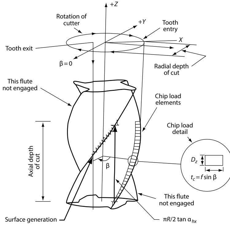
FIGURE 8.6 Uncut chip area in end milling. (After Kline, W.A., and DeVor, R.E., Int. J. MTDR , 23, 123, 1983.)
