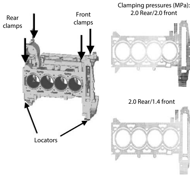
FIGURE 8.30 Analytical study of varying clamping pressures to control flatness in engine block deck milling. (From Stephenson, D.A., Casting and Machining Process Analysis at GM Powertrain, SAE Technical Paper 2002-01-0622, 2002.)
