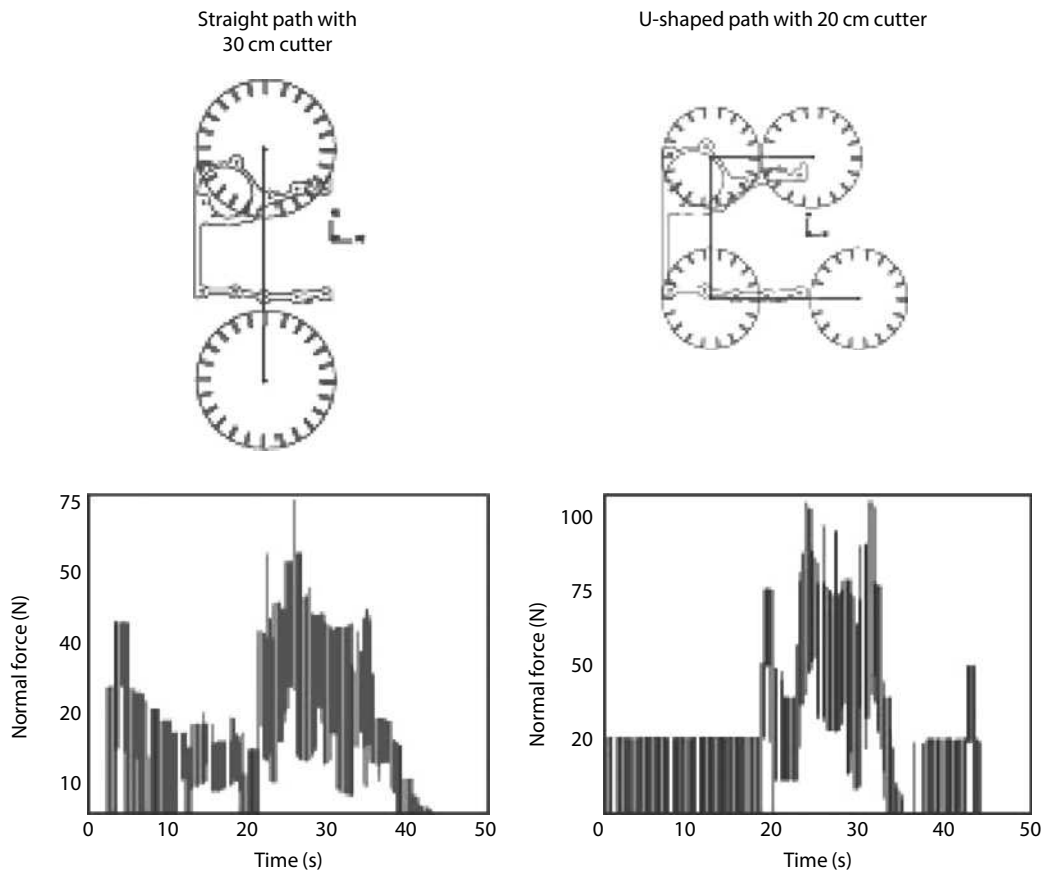
FIGURE 8.20 Analysis of two options for milling an engine block front face. (From Stephenson, D.A., Casting and Machining Process Analysis at GM Powertrain , SAE Technical Paper 2002-01-0622, 2002.) (a) Large cutter with straight path and (b) small cutter with U-shaped path. For a fixed cycled time, case (a) yields 30% better flatness accuracy than case (b), since the shorter tool path permits use of a lower feed rate, resulting in lower forces normal to the cut surface.
