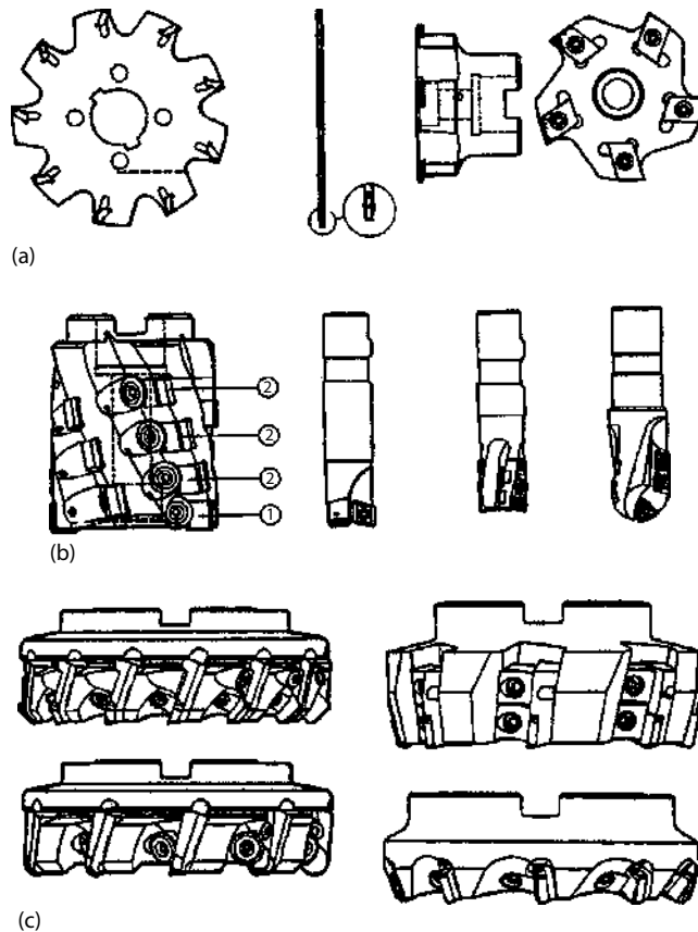
FIGURE 4.34 Indexable milling cutters. (a) Slot milling, (b) slot- and contour-milling, and (c) face milling. (Courtesy of Carboloy/Seco, Warren, MI.)
