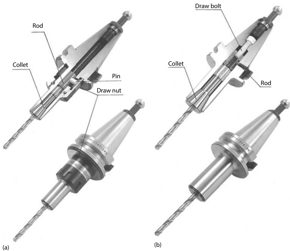
FIGURE 5.58 Extended positive pull-collet designs for extended toolholders with a 2 mm chucking range. (a) Draw nut design and (b) draw bolt design. (Courtesy of Tecnara Tooling Systems, Inc., Santa Fe Springs, CA.)
