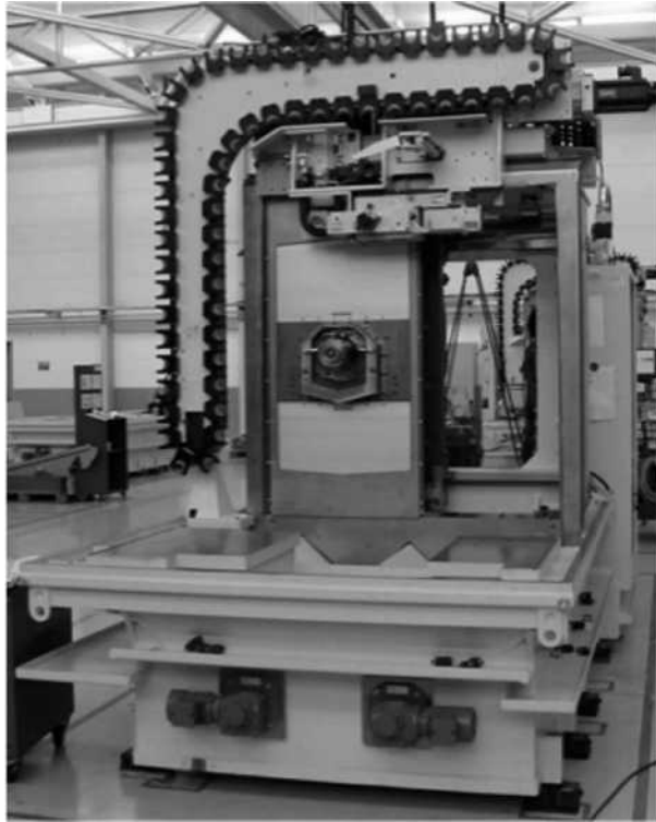
FIGURE 3.63 Chain tool magazine on a horizontal machining center. (Courtesy of MAG Automotive, Sterling Heights, MI.)
