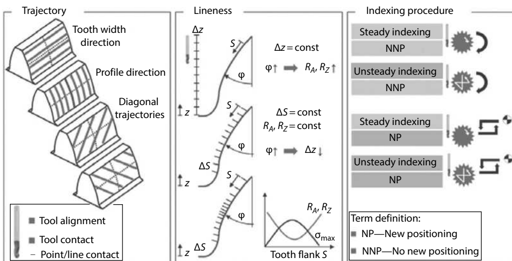
FIGURE 17.22 Elements of machining strategies for free-form milling of gears. (After Klocke et al. [109].)
