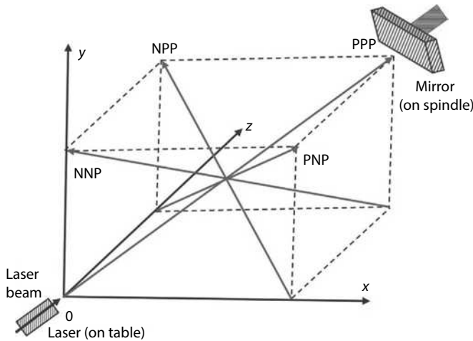
FIGURE 16.18 Schematic of the four body diagonals method to evaluate the volumetric accuracy of the workspace.
