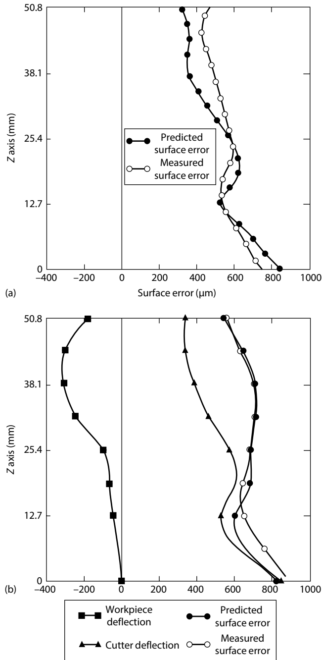
FIGURE 8.27 Surface errors in end milling of aluminum with a high-speed steel cutter: (a) rigid workpiece; (b) compliant workpiece. (After Kline, W.A. et al., Int. J. MTD , 22, 7, 1982.)
