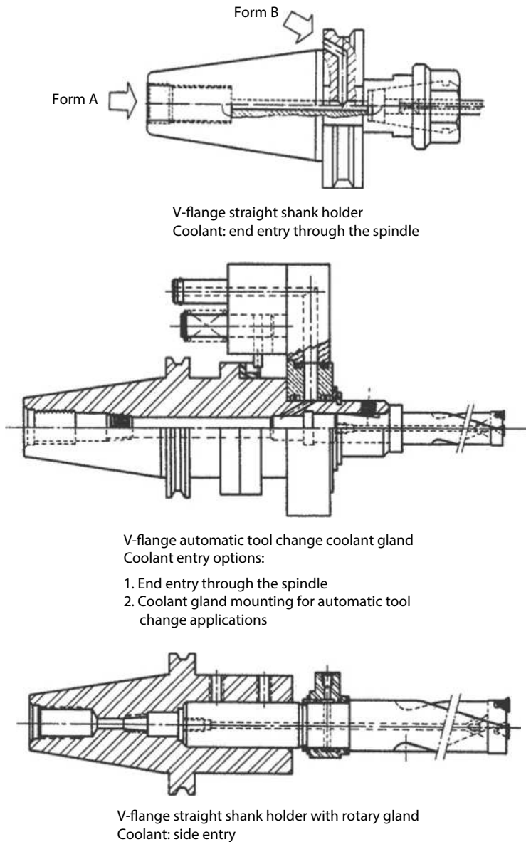
FIGURE 5.52 Typical coolant toolholder adapters for coolant-fed rotary cutting tools. (Courtesy of The George Whalley Company, Cleveland, OH.)
