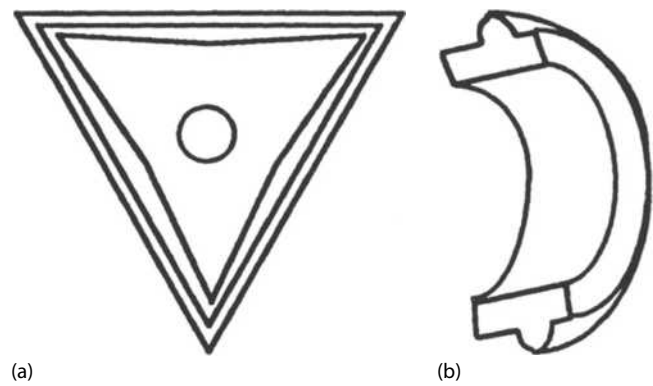
FIGURE 11.7 (a) Insert with formed-in chip breaking groove. (b) Chip with thickened section produced by grooved insert. (After Kaldor, S. et al., ASME J. Eng. Ind. , 101, 241, 1979.)
