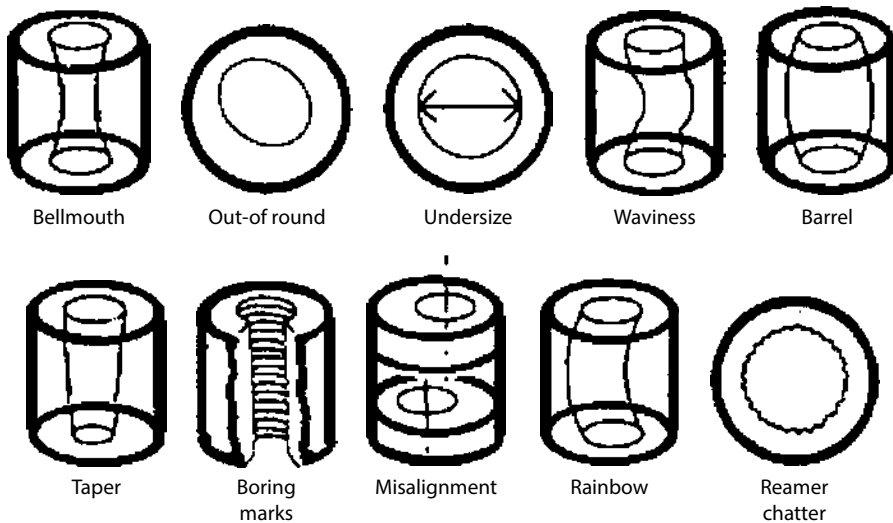
FIGURE 2.32 Bore form and size errors corrected by microfinishing or honing.
