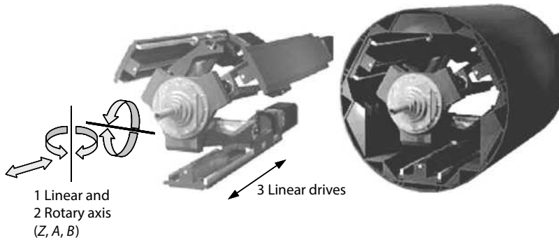
FIGURE 3.40 The structural configuration of the Sprint-Z3 spindle on parallel mechanism (3DOF PKM with three fixed length struts). This 3DOF head is used in a five-axis machine with X- and Y-axis with conventional drives on the head or workpiece carrier. (From DST Machine GmbH, Mönchengladbach, Germany.)
