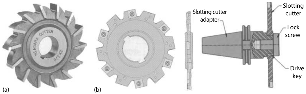
FIGURE 2.39 Comparison of slot milling cutters: (a) using an edge across the full width of the slot and (b) a staggered tooth cutter. (Courtesy of Kennametal and Carboloy, Latrobe, PA.)
