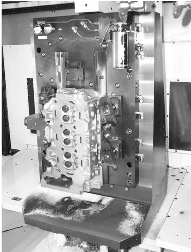
FIGURE 5.88 Typical tombstone-type CNC fixture for an engine head. (From General Motors Corporation, Detroit, MI.)
