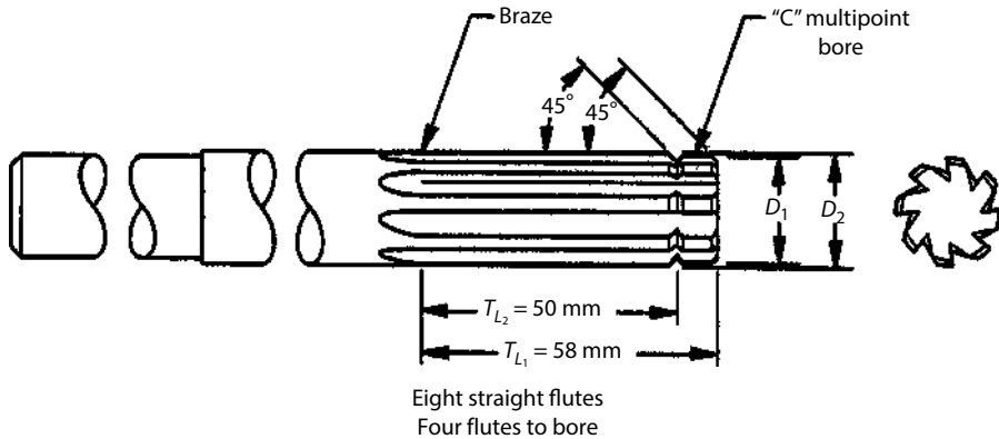
FIGURE 4.81 Configuration of a bore-reaming tool.
