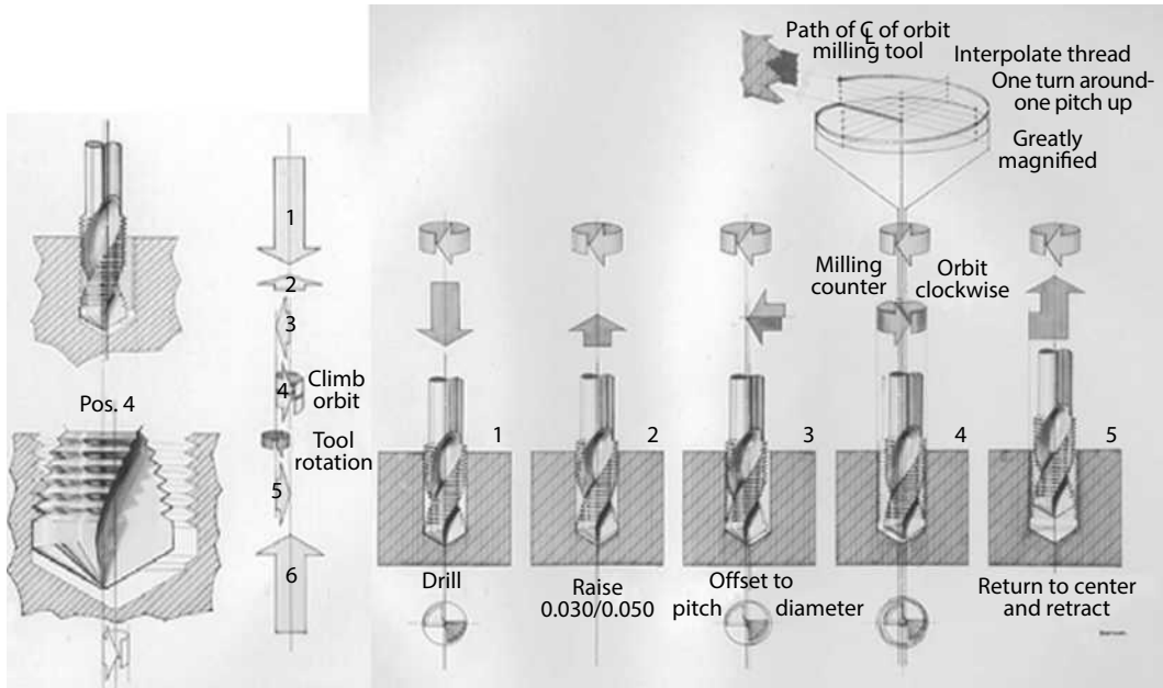
FIGURE 2.25 Drill/threadmilling using a combination drill and thread milling tool.
