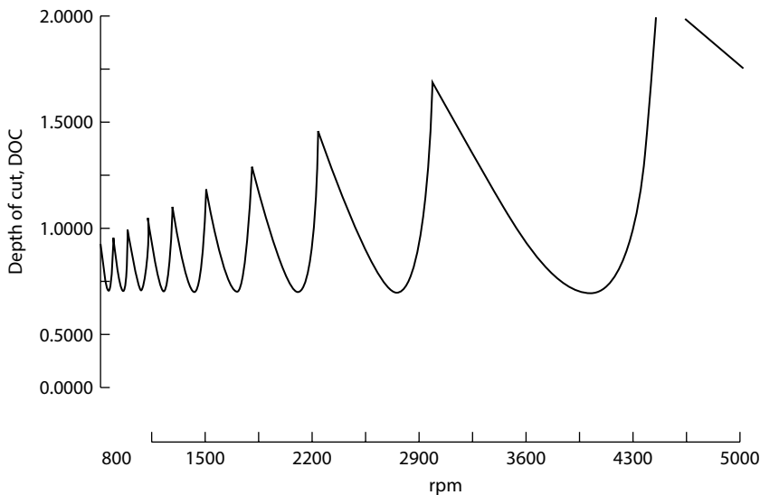
FIGURE 12.54 Stability lobe diagram for the modified spindle with a boring tool installed on the machine.
