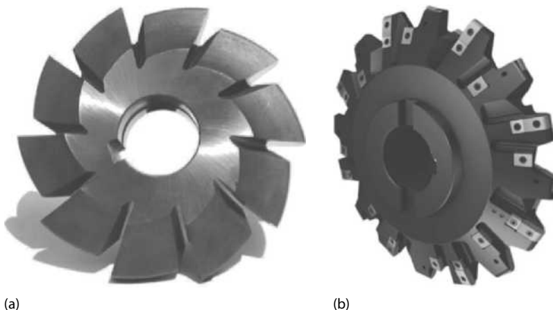
FIGURE 17.10 Disk-type form milling cutters: (a) solid HSS and (b) indexable carbide.
