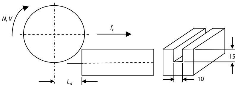
FIGURE 2.38 Schematic representation of Example 2.8.
