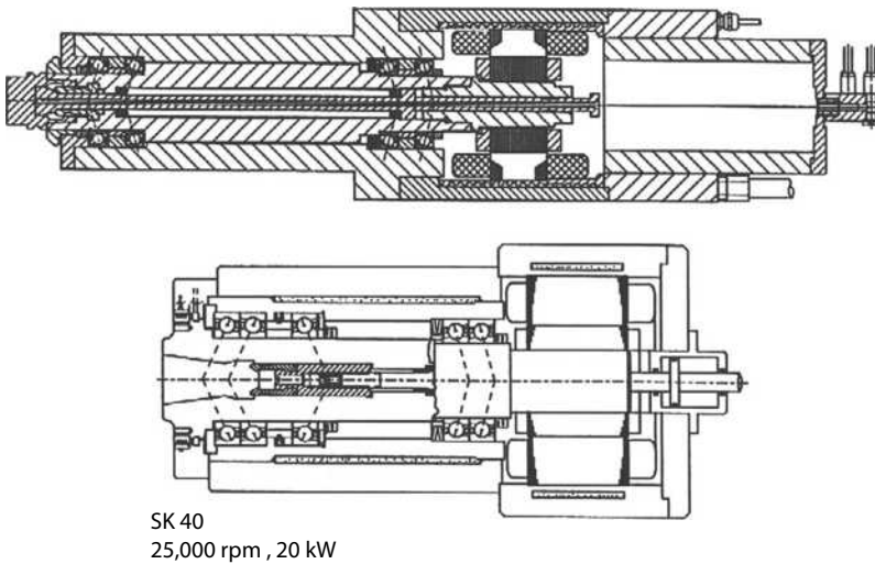
FIGURE 3.53 Motorized spindles with “flywheel” motor arrangement. (Courtesy of the Precise Corporation, Racine, WI.)
