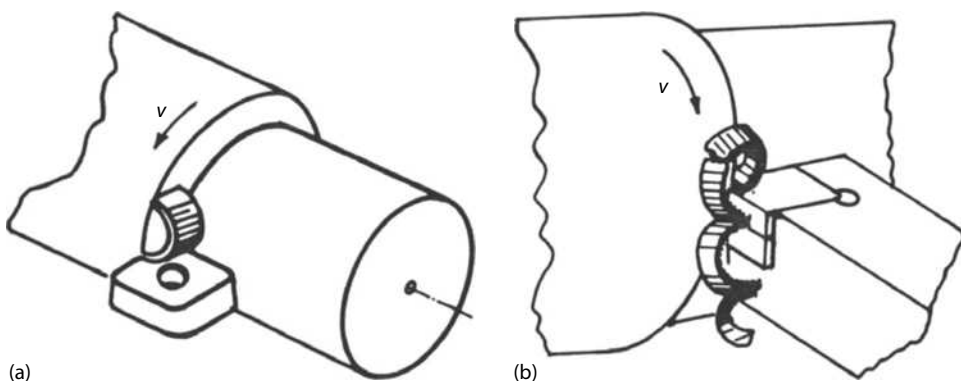
FIGURE 11.4 Breaking of the chip against the workpiece surface (a) or tool holder (b). (After Kaldor, S. et al., ASME J. Eng. Ind. , 101, 241, 1979.)
