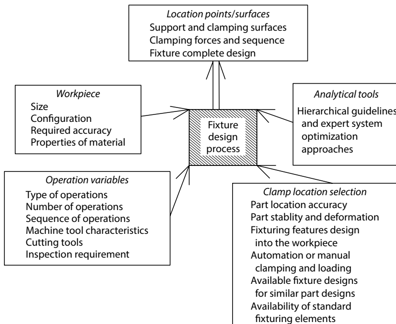
FIGURE 5.84 Factors influencing the design of a fixture.
