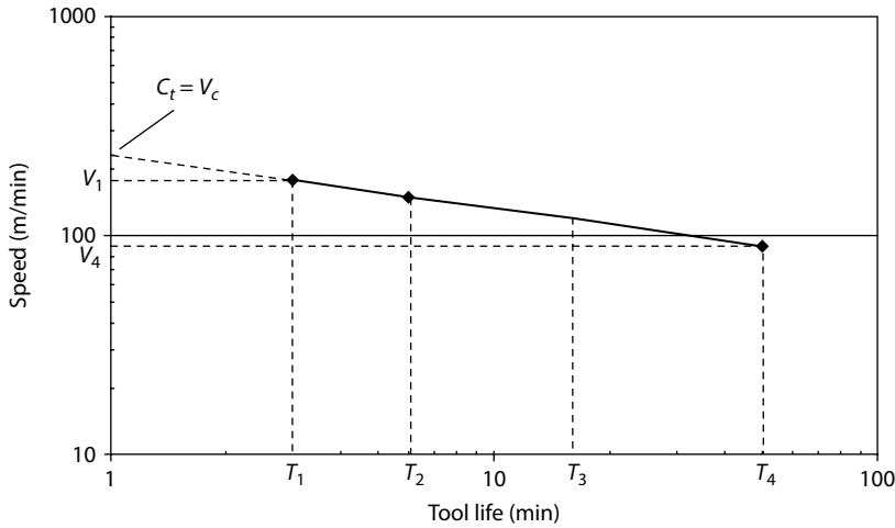
FIGURE 9.31 Log-log plot of tool life versus cutting speed for Example 9.1.
