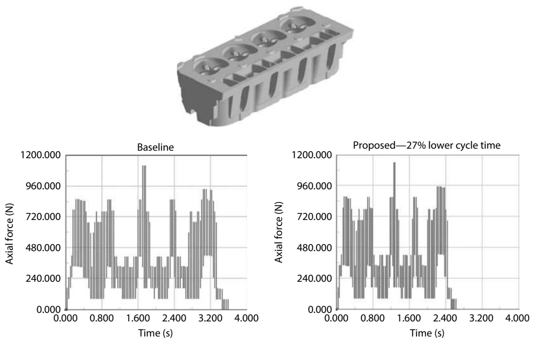
FIGURE 8.23 Axial force plots for baseline and proposed tool paths and milling cutters for an engine head cubing operation. (From White, D.R., Machining Applications at GM Powertrain , Proceedings of 2002 Third Wave AdvantEdge User's Conference , Atlanta, GA, April 2002, Paper 6.)
