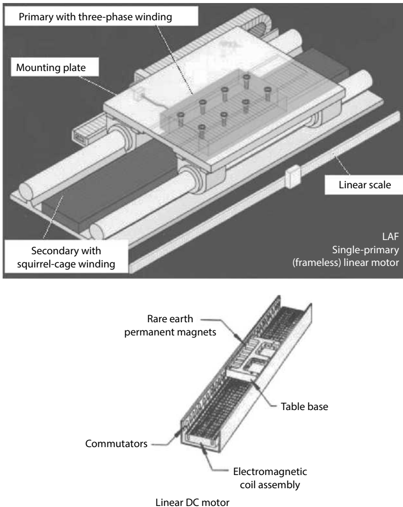
FIGURE 3.48 Linear axis drive motors. (Courtesy of The Rexroth Corporation, Indramat Division, Rochester Hills, MI.)
