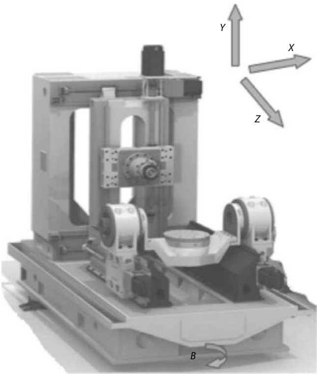
FIGURE 3.16 Horizontal spindle five-axis machining center with a B-axis table mounted on an A-axis trunnion. (Courtesy of MAG Automotive, Sterling Heights, MI.)
