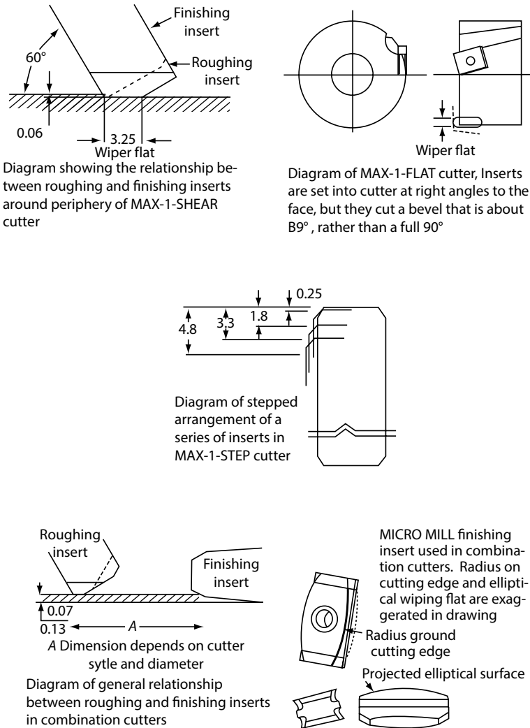
FIGURE 4.45 Diagram showing the relationship between roughing and finishing inserts in a combination milling cutter. (Courtesy of Ingersoll Cutting Tool Division, Rockford, IL.)
