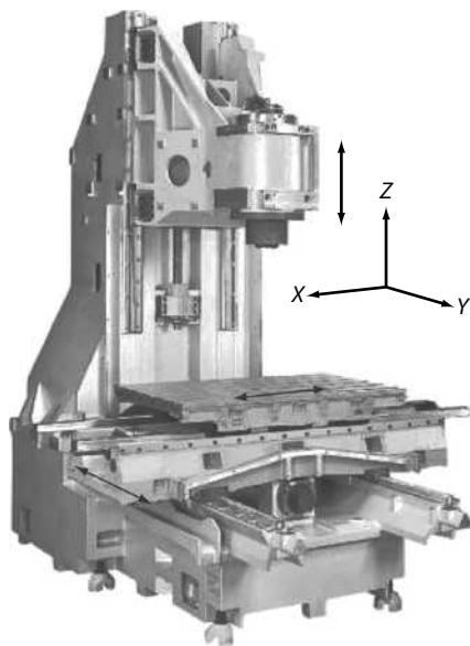
FIGURE 3.11 Solid base, fixed column vertical spindle three-axis machining center with Z-axis travel (vertical movement on spindle head), X-axis travel (longitudinal movement of table), and Y-axis travel (cross movement of saddle). (Courtesy of Mori Seiki Co., Ltd., Nagoya, Japan.)
