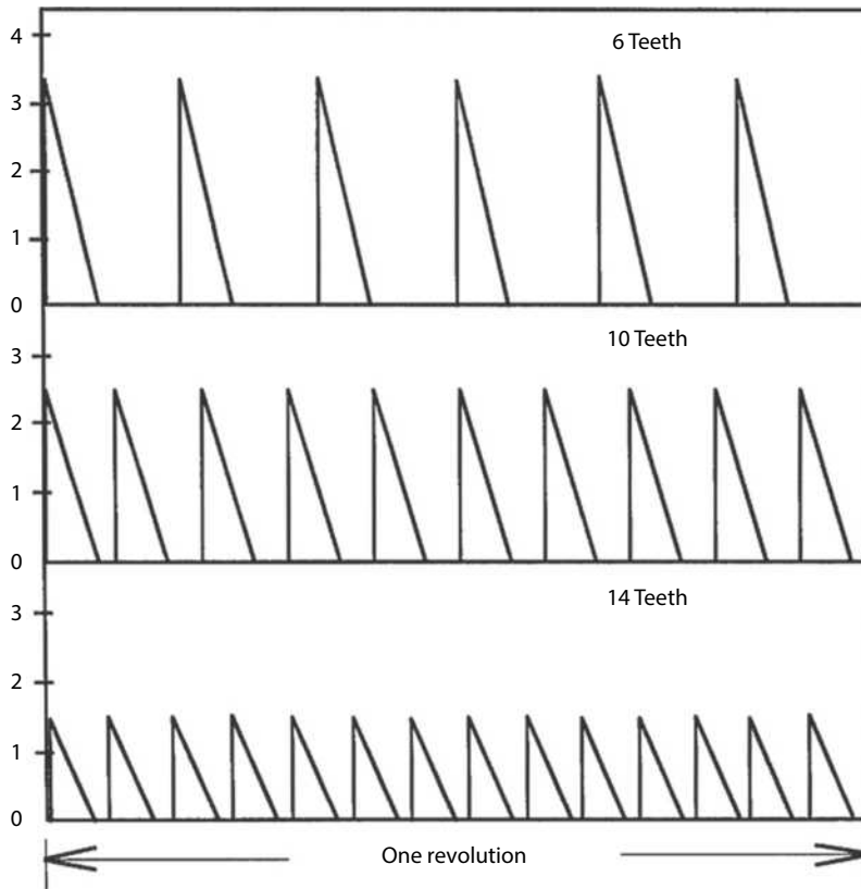
FIGURE 12.11 Variations in spindle torque or forces during climb (down) milling with a zero axial and radial rake cutter.
