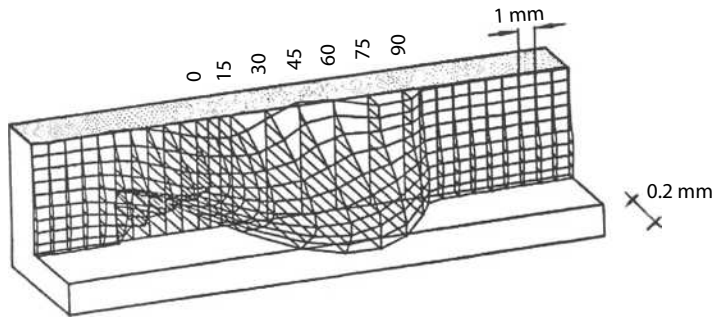
FIGURE 8.9 Simulated surface error in a pocketing cut in end milling. (After Tlustý, J., Effect of end milling deflections on accuracy, Handbook of High Speed Machining Technology , Chapman & Hall, New York, 1985, pp. 140–153.)
