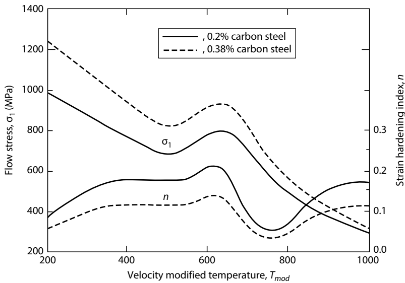
FIGURE 6.32 Variation of \sigma and n with T_{mod} for two plain carbon steels. (After Oxley, P.L.B., The Mechanics of Machining , Ellis Horwood, Chichester, U.K., 1989.)
