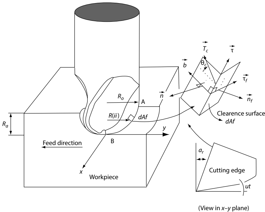
FIGURE 8.10 Uncut chip area in ball end milling. (After Yucesan, G., and Altintas, Y., Mechanics of Ball End Milling Process , Manufacturing Science and Engineering , ASME PED Vol. 64, ASME, New York, 1993, pp. 543–551.)
