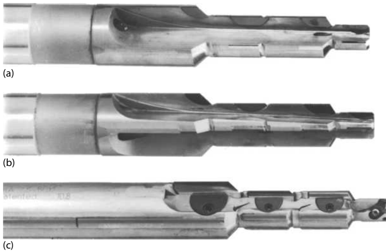
FIGURE 4.79 Configurations of reamers for short and deep holes. (a) Multistep PCD tip gun reamer, (b) multistep, mult flute PCD tip reamer, and (c) multistep inserted blade gun reamer.
