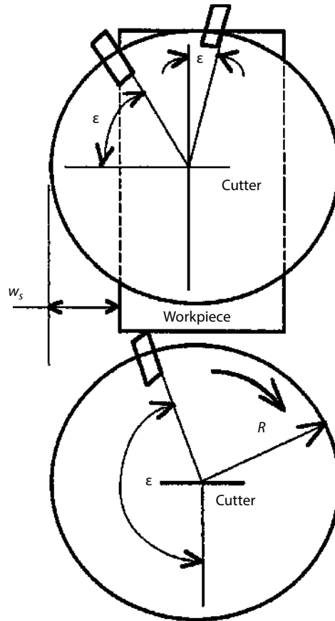
FIGURE 4.43 Schematic view of initial cutting edge contact at the entrance of a workpiece. (Courtesy of Carbology/Seco, Warren, MI.)
