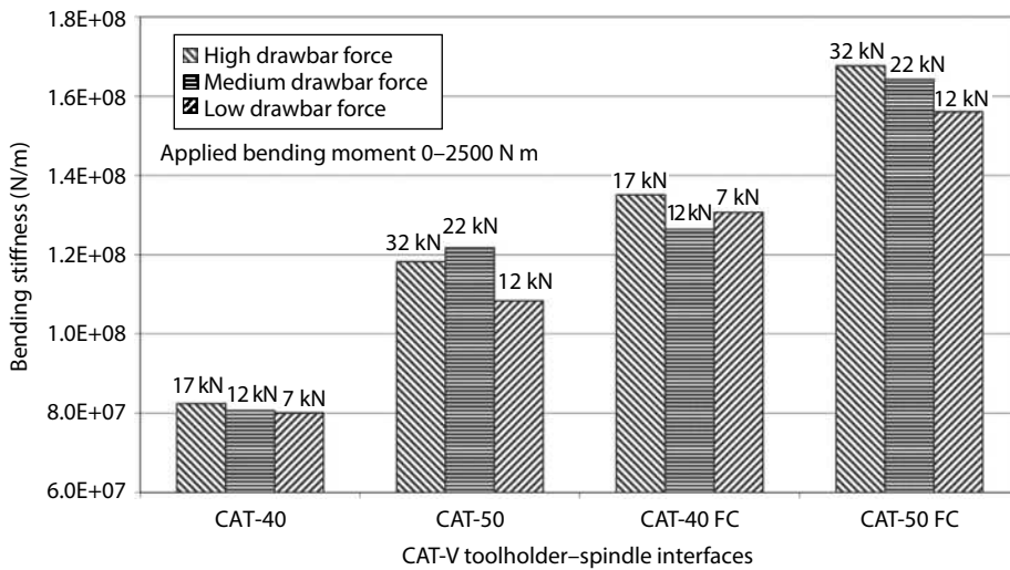
FIGURE 5.18 Effect of drawbar preload on static bending stiffness for various interfaces.
