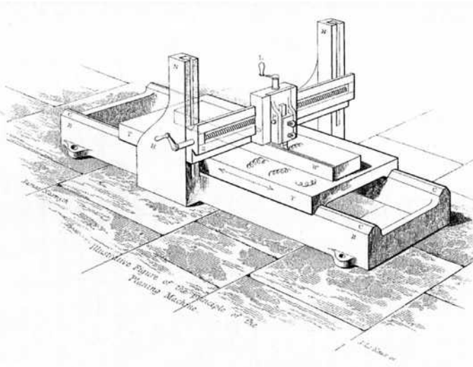
FIGURE 1.10 Typical early English planer. (From Naysmith, J., Remarks on the Introduction of the Slide Principle in Tools and Machines Employed in the Production of Machinery, in R. Buchanan, Ed., Practical Essays on Millwork and Other Machinery , 3rd edn., John Weale, London, U.K., 1841, Appendix B, pp. 393–418.)
