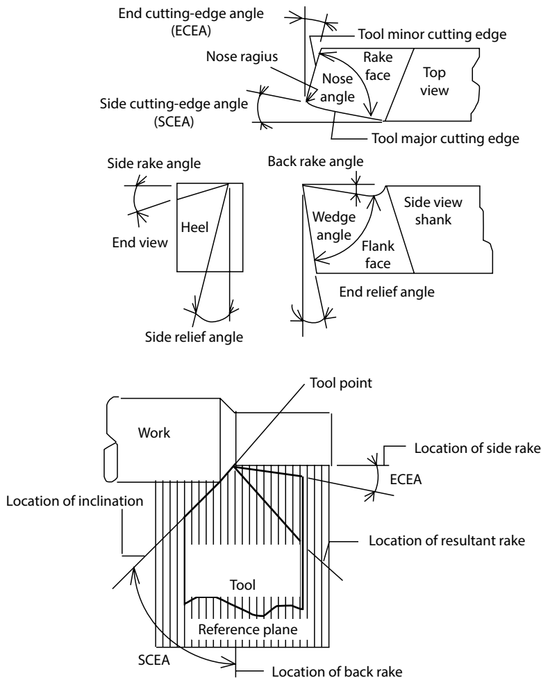
FIGURE 4.16 Standard terminology to describe the basic geometry of single-point tools.
