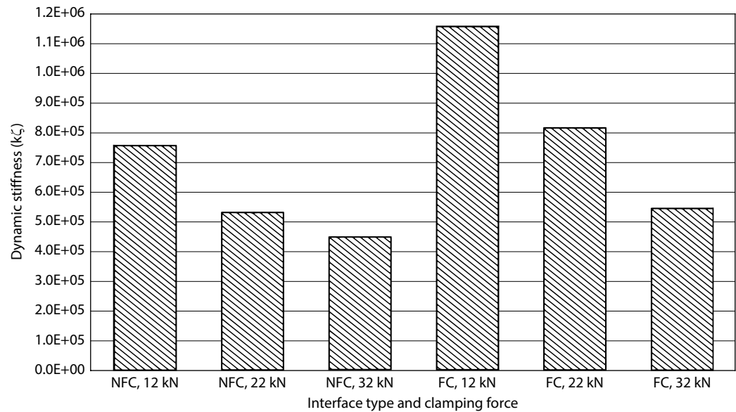
FIGURE 5.31 Comparison of dynamic bending stiffness for CAT-V with (FC) and without (NFC) face contact interface shown in Figure 5.30.
