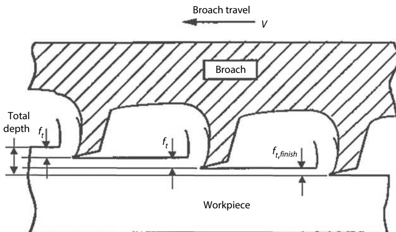
FIGURE 2.18 Broaching.
