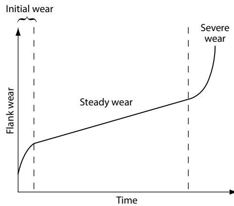
FIGURE 9.4 Variation of the flank wear rate with cutting time, showing the initial wear, steady wear, and severe wear periods.
