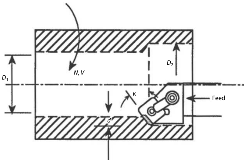
FIGURE 2.3 Boring.
