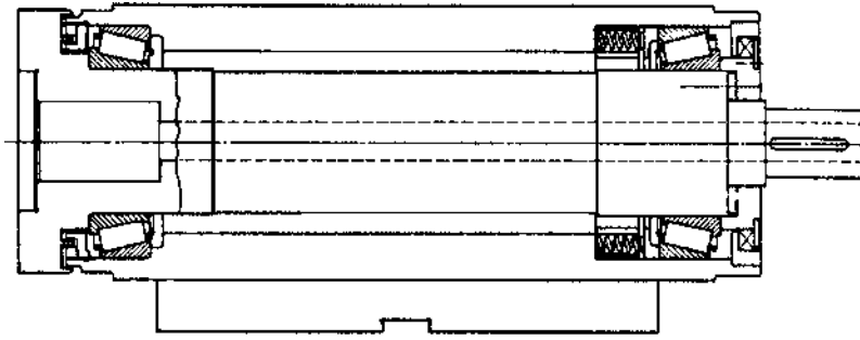
FIGURE 3.59 Spindle with tapered roller bearings (grease lubrication). (Courtesy of Timken Company, Canton, OH.)
