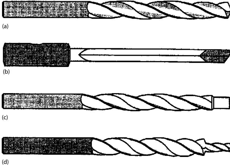
FIGURE 4.48 Regrindable drill types. (a) Regular drill, (b) gun drill, (c) pilot drill, and (d) counter drill.
