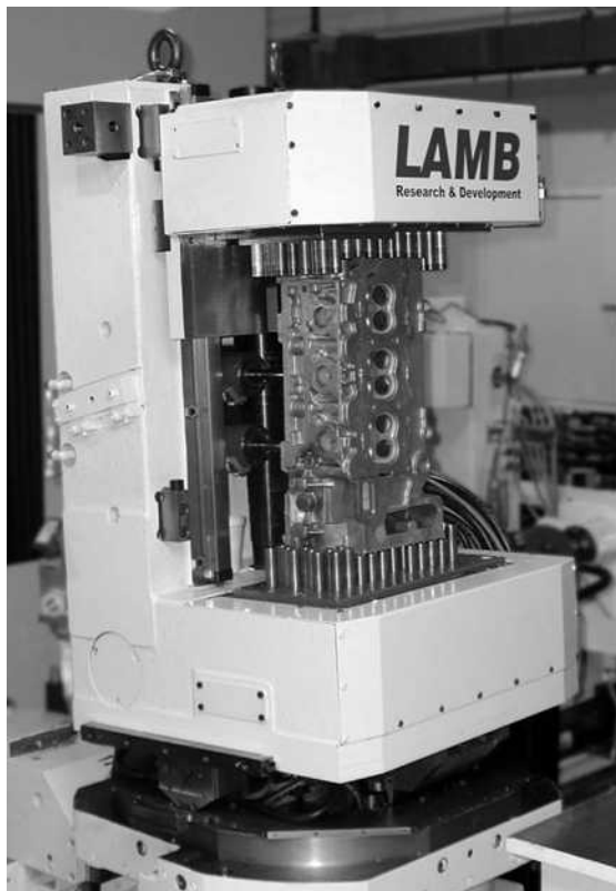
FIGURE 5.94 Bed of Nails fixture shown holding an engine head. (From Lamb Technicon, Warren, MI.)
