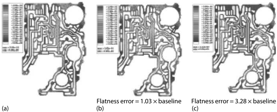
FIGURE 8.29 Analysis to determine the sensitivity of part flatness to locating and fixturing errors when finish milling a channel plate. (a) Baseline, (b) Center locators missing, and (c) Top clamp and center locators missing. (From Stephenson, D.A., Casting and Machining Process Analysis at GM Powertrain, SAE Technical Paper 2002-01-0622, 2002.)
