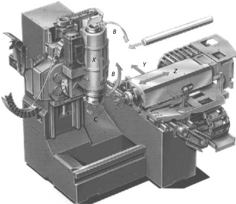
FIGURE 3.18 Five-axis bar machining center capable of five-sided machining with one clamping. The Y - and Z -axis motions are provided by the table while the X -axis motion is performed by the column. The workpiece carrier has a B -axis with a swiveling range of 270^\circ and a C -axis with a swiveling range of 360^\circ . (Courtesy of Hermle Machine Company LLC, Franklin, WI.)
