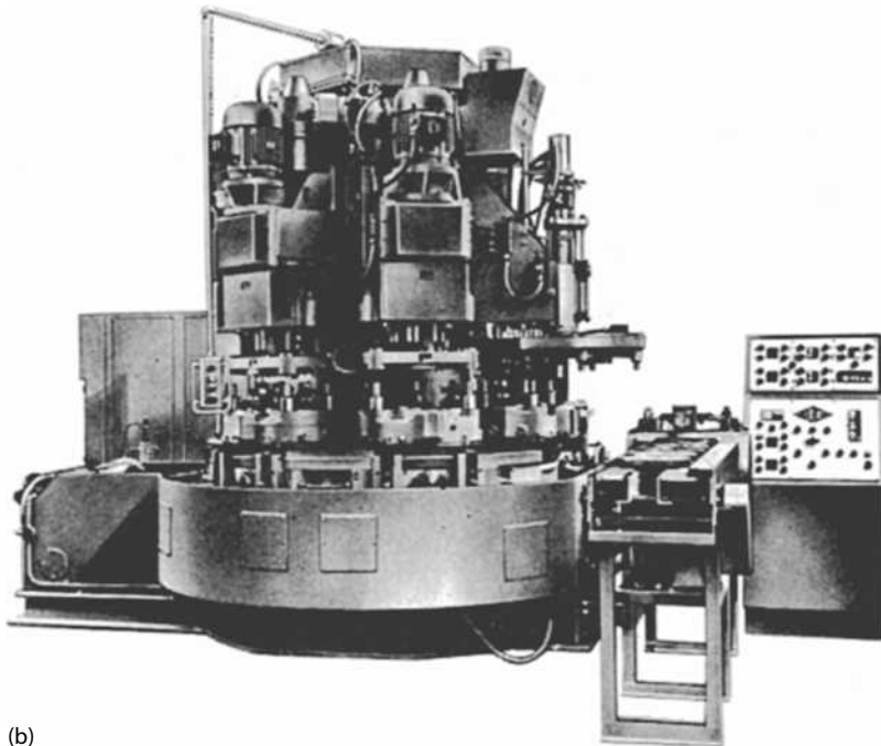
FIGURE 3.1 Rotary transfer machines. (a) Rotary indexing system. (From Moss Group Automation, Annesley, Nottingham, U.K.) (b) Center column system. (After Charman, B.W., Special Purpose Production Machines , Crosby Lockwood & Son Ltd., London, U.K., 1968.)
