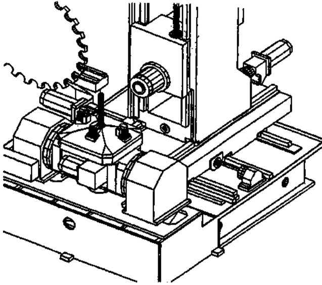
FIGURE 3.17 A five-axis machine using an integral tilt trunnion rotary table with 150^\circ of motion on the A -axis ( +30^\circ to -120^\circ ) combined with a B -axis.
