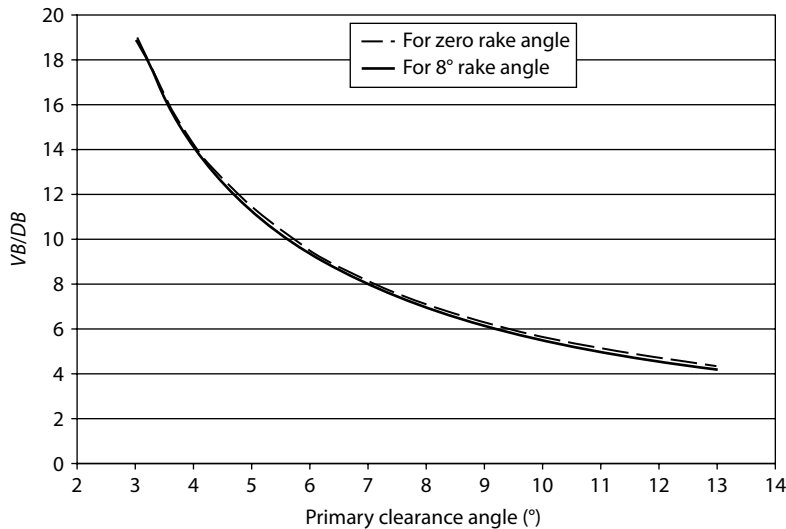
FIGURE 9.34 Relationship between the width of flank wear land VB and the clearance angle for zero and 8^\circ rake tools for the data in Example 9.3.
