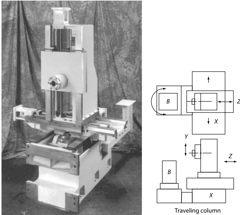
FIGURE 3.33 Structural components of a three- or four-axis horizontal spindle machining center with traveling column and either fixed or rotary table. All X-, Y-, and Z-axis motions are provided in the column. (Courtesy of Cellular Concepts, Detroit, MI.)
