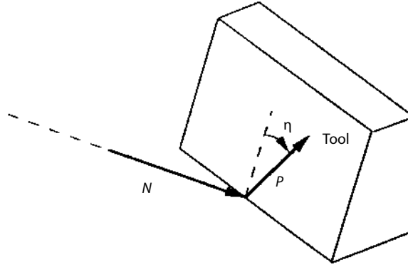
FIGURE 6.4 The forces N and P on the rake face of an oblique cutting tool.
