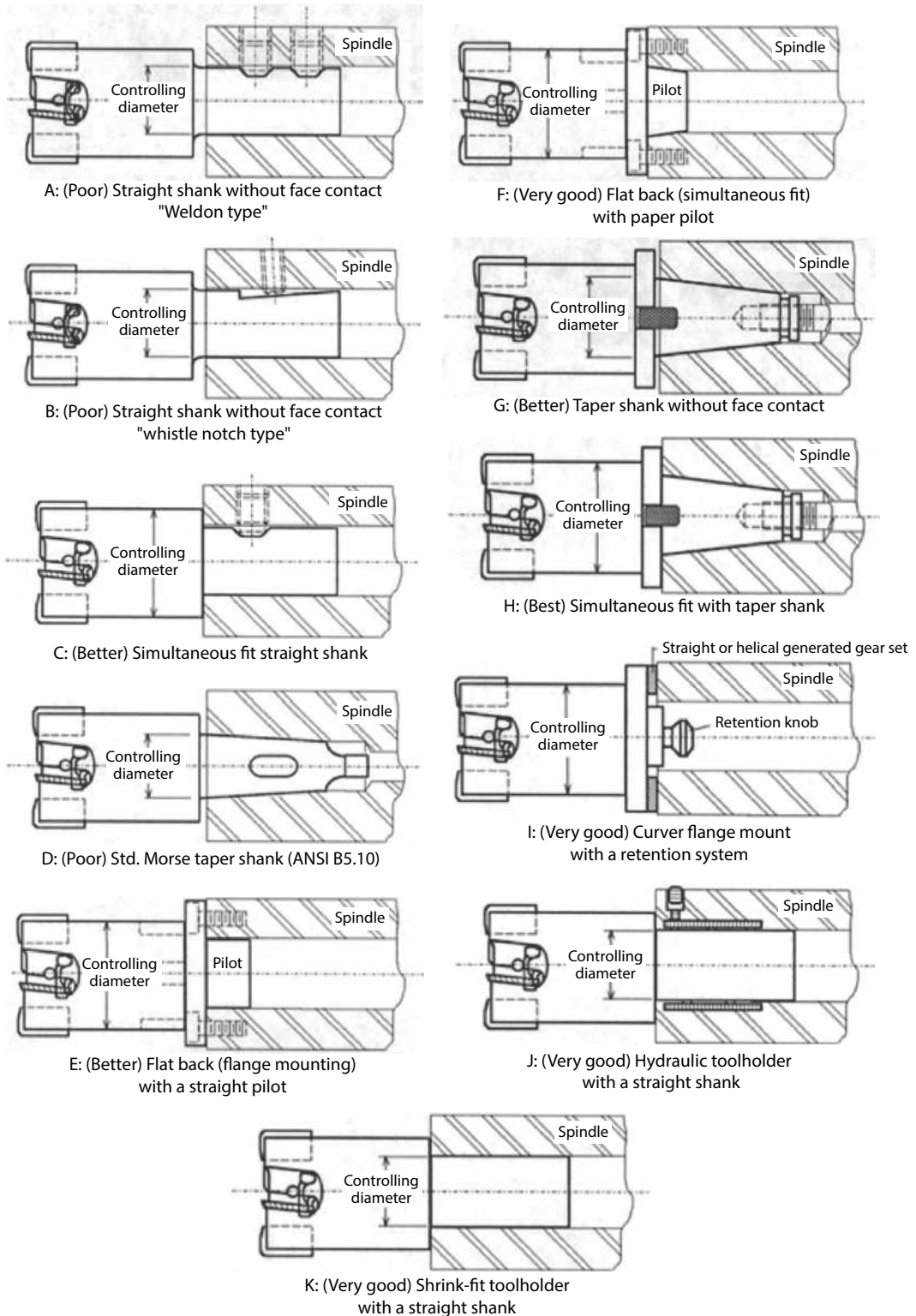
FIGURE 5.11 Spindle-toolholder connections.
