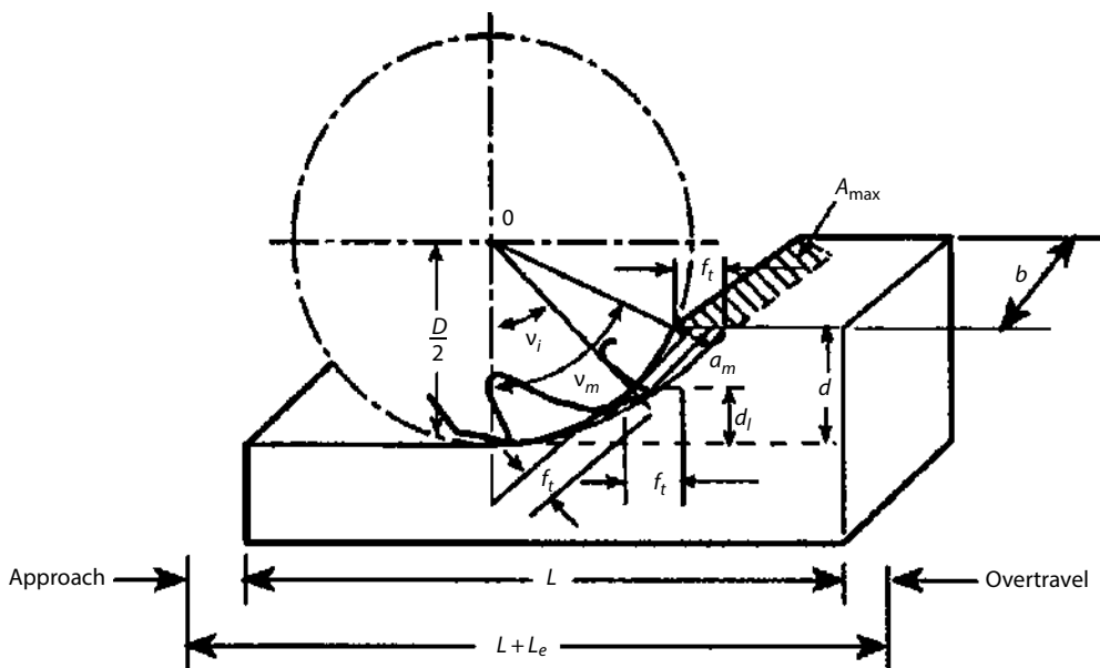
FIGURE 2.14 Characteristics of peripheral (or plain) milling.
