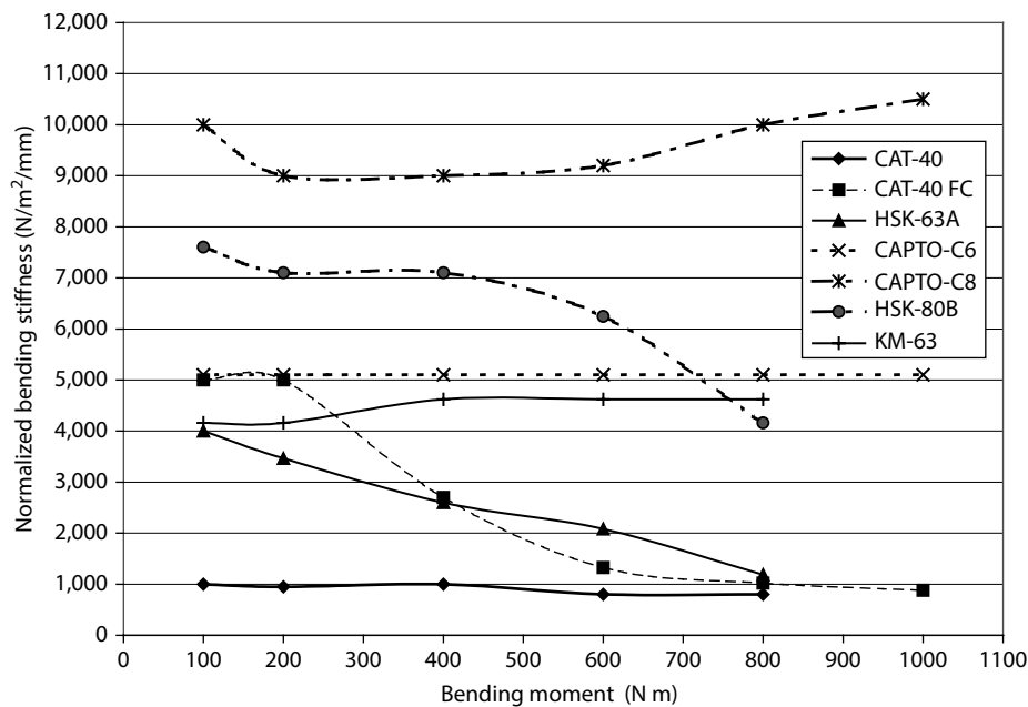
FIGURE 5.22 Normalized static bending stiffness for various small interfaces.
