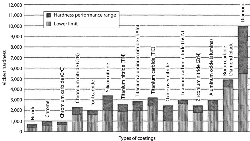
FIGURE 4.11 Comparison of microhardness for several types of coatings.
