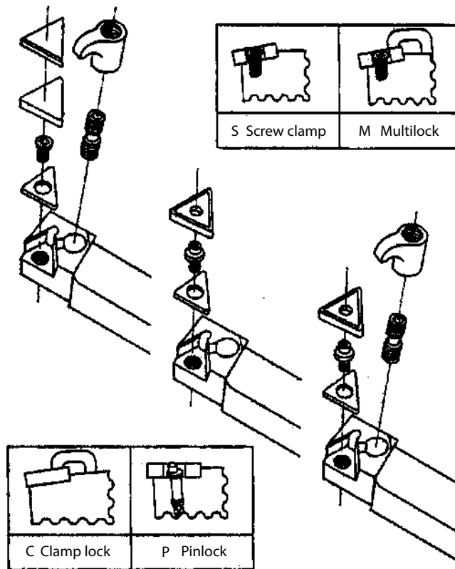
FIGURE 4.22 Basic insert locking (holding) methods. (Courtesy of Carboloy/Seco, Warren, MI, and Sumitomo Electric Corp., Osaka, Japan.)
