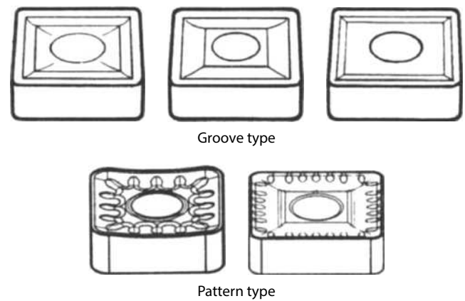
FIGURE 11.6 Typical chip breaking patterns formed into inserts.
