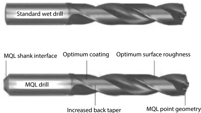
FIGURE 15.17 Differences in drill geometries between wet and MQL drills. MQL drills also commonly have larger, polished flutes for chip evacuation. (From Minimale Mengenschmierung-Grundlagen , Gühring KG, Albstadt, Germany, 2013.)
