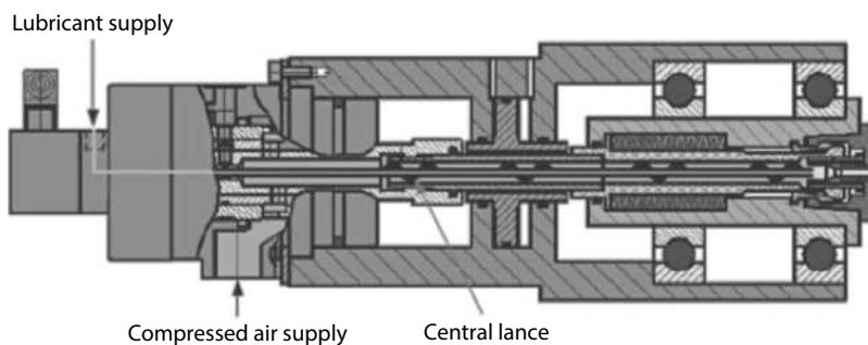
FIGURE 15.9 Rotary union and spindle modifications required for two-channel MQL in through-tool delivery applications. (From Handbuch Minimalmengenschmierung [MMS], KometGroup GmbH, Besigheim, Germany, March 2008.)
