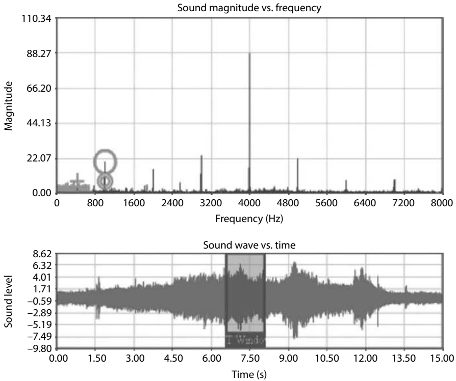
FIGURE 12.39 Audio signal of a vibration case using a 30 inserts PCD face mill in Example 12.4. (Harmonizer® Courtesy of Manufacturing Laboratories Inc., Las Vegas, Nevada.)
