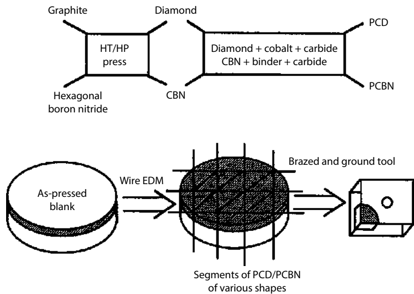
FIGURE 4.9 Manufacturing process for PCD/PCBN inserts.
