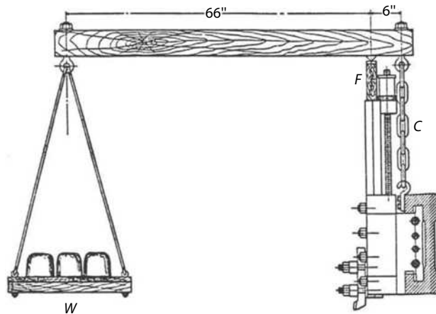
FIGURE 1.19 Balance beam dynamometer for measuring the feed force on a boring mill. W is the counter-weight, F is the fulcrum for the 11:1 lever arm, and C is the chain to the tooling assembly. (From Taylor, F.W., ASME Trans. , 28, 31, 1906.)
