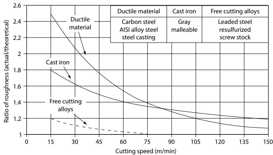
FIGURE 10.13 Variation of measured roughness with cutting speed. (Data courtesy of Carboloy Inc., Warren, MI.)
