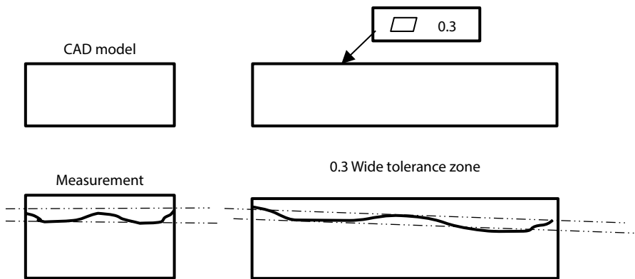
FIGURE 10.23 Illustration of surface flatness.
