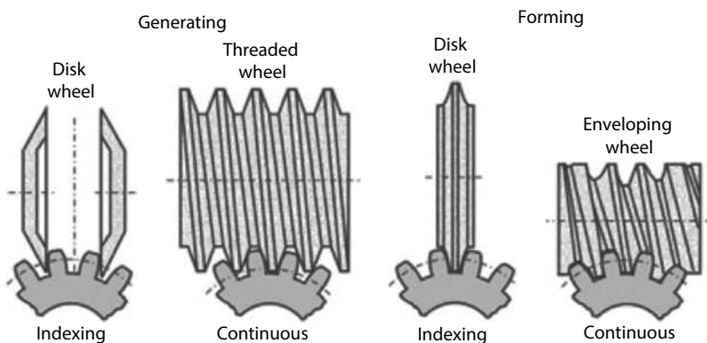
FIGURE 17.27 Cylindrical gear grinding processes.
