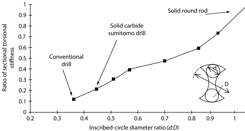
FIGURE 4.50 Effect of web thickness on drill's torsional stiffness. (From Rigidity of Twist Drills , Metal Cuttings , 10(3), National Twist Drill and Tool Company, Rochester, MI, July 1962; Skoglund, J., Cutting Tool Eng. , 35, February 1990.)
