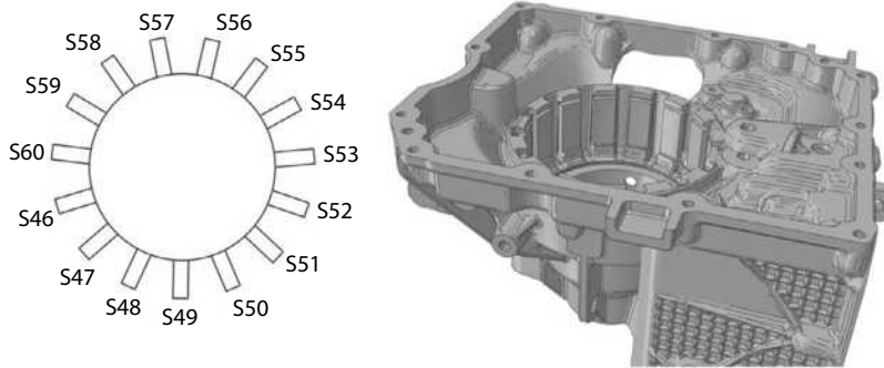
FIGURE 16.41 Machined slots in a transmission converter housing.
