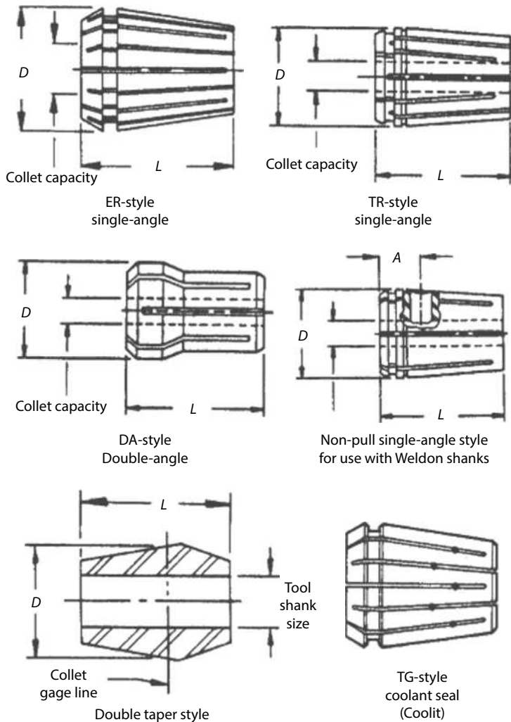
FIGURE 5.57 Collet types.
