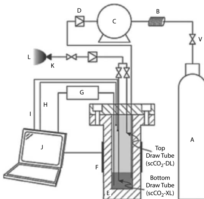
FIGURE 15.20 Schematic of supercritical CO 2 MQL delivery system. (A) Cylinder of food-grade CO 2 , (B) cooling unit, (C) pump, (D) check valve, (E) high pressure vessel, (F) heating element, (G) soybean oil sump, (H) pressure transducer, (I) thermocouple, (J) computer, (K) nozzle, (L) supercritical CO 2 MQL spray, (V) on/off valve. (After Supekar, S.D., J. Mater. Process. Technol. , 212, 2652, 2012.)
