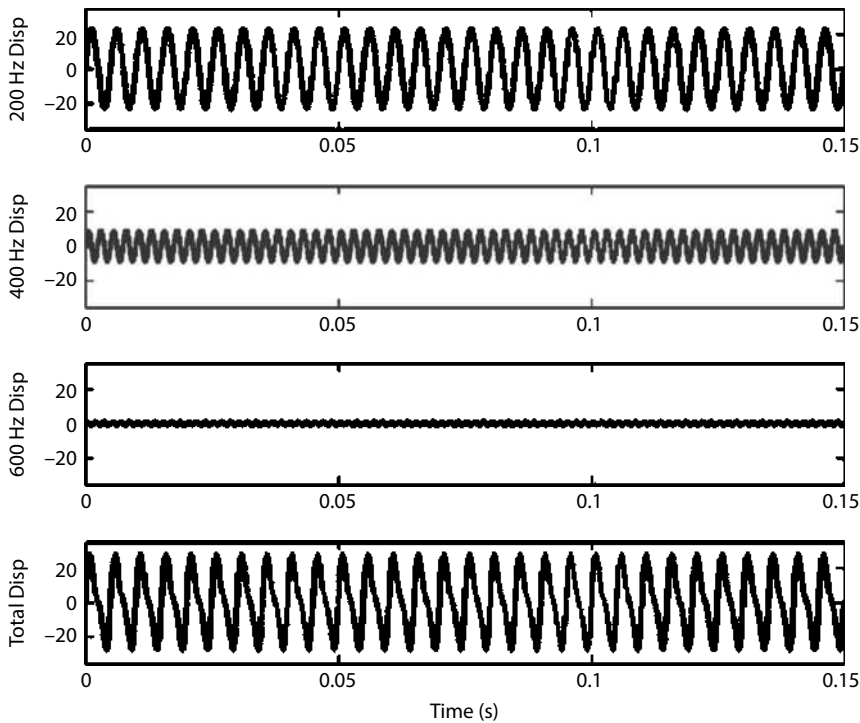
FIGURE 12.36 Time domain for the 6000 rpm displacement ( \mu\text{m} ) for the FRF of part in Figure 12.35. (Courtesy of D3 Vibrations Inc.)
